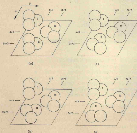
FIG. 1. Projections of the structure on (001); (a), (b), (c), and (d) show the four orientations of molecule II (see Table II).
